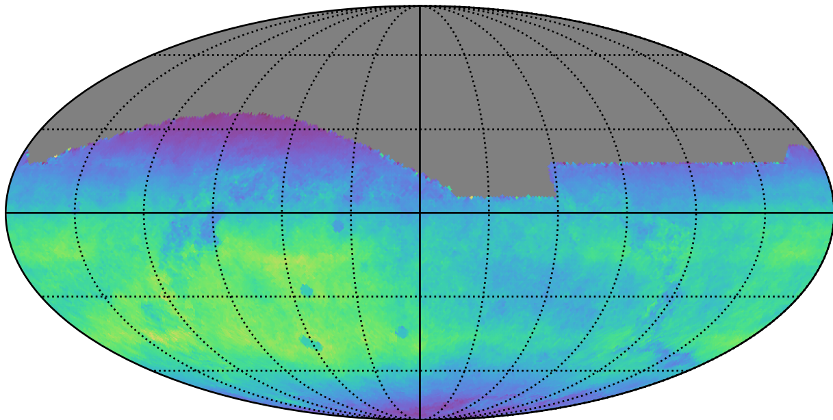
all_long_v3.4_10yrs All sky r band: Normalized Teff
