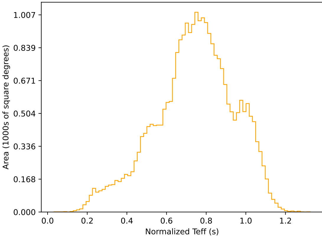
all_long_v3.4_10yrs All sky r band: Normalized Teff
