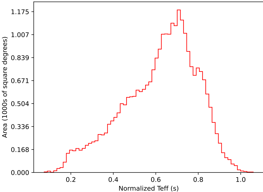
all_long_v3.4_10yrs All sky i band: Normalized Teff
