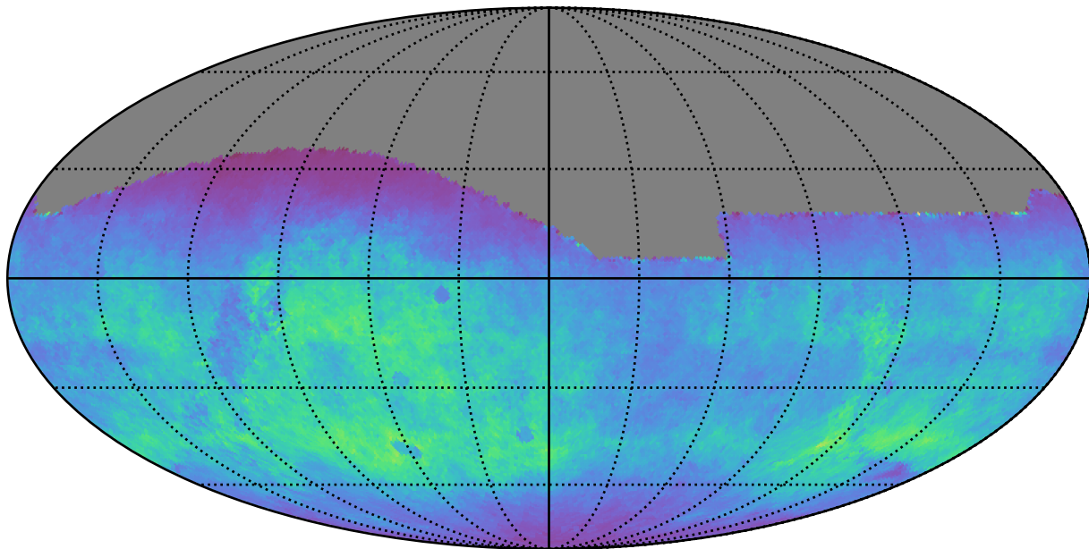
all_long_v3.4_10yrs All sky g band: Normalized Teff
