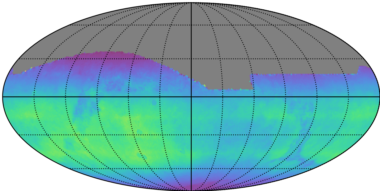
all_long_v3.4_10yrs All sky all bands: Normalized Teff
