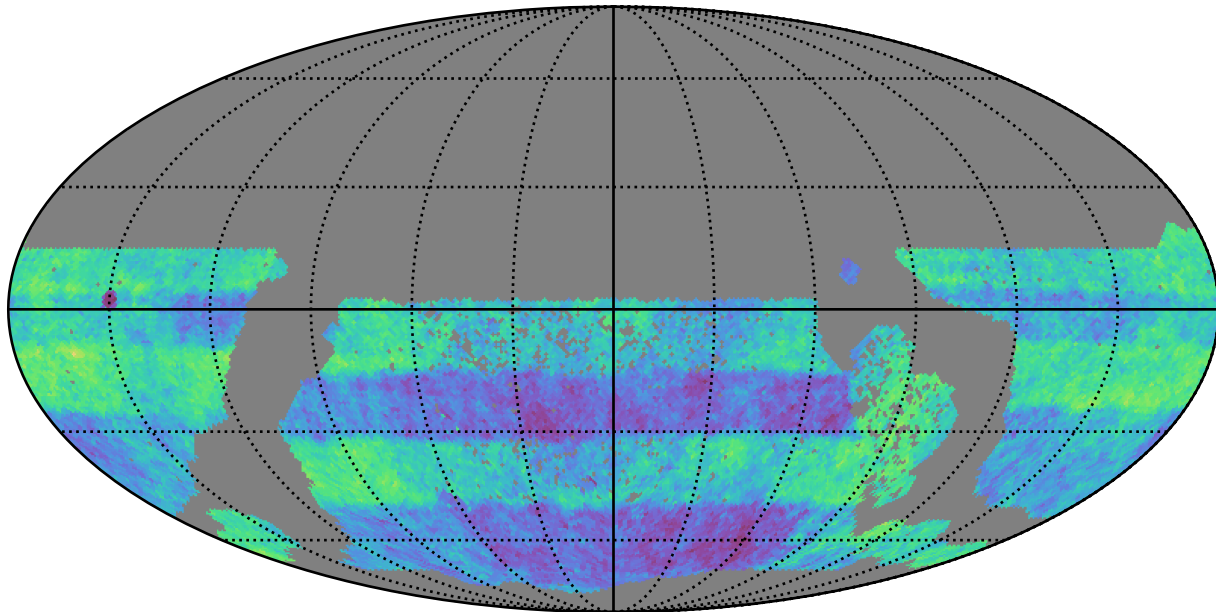
all_long_v3.4_10yrs WFD: Normalized Proper Motion Uncert @ 24.0
