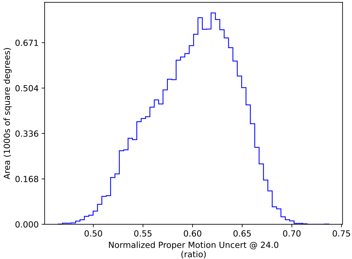
all_long_v3.4_10yrs WFD: Normalized Proper Motion Uncert @ 24.0
