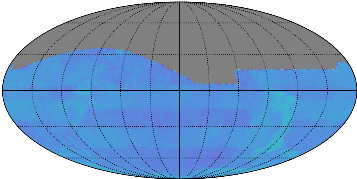
all_long_v3.4_10yrs All sky: Normalized Proper Motion Uncert @ 24.0
