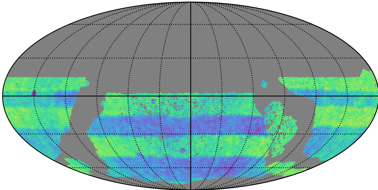
all_long_v3.4_10yrs WFD: Normalized Proper Motion Uncert @ 20.5
