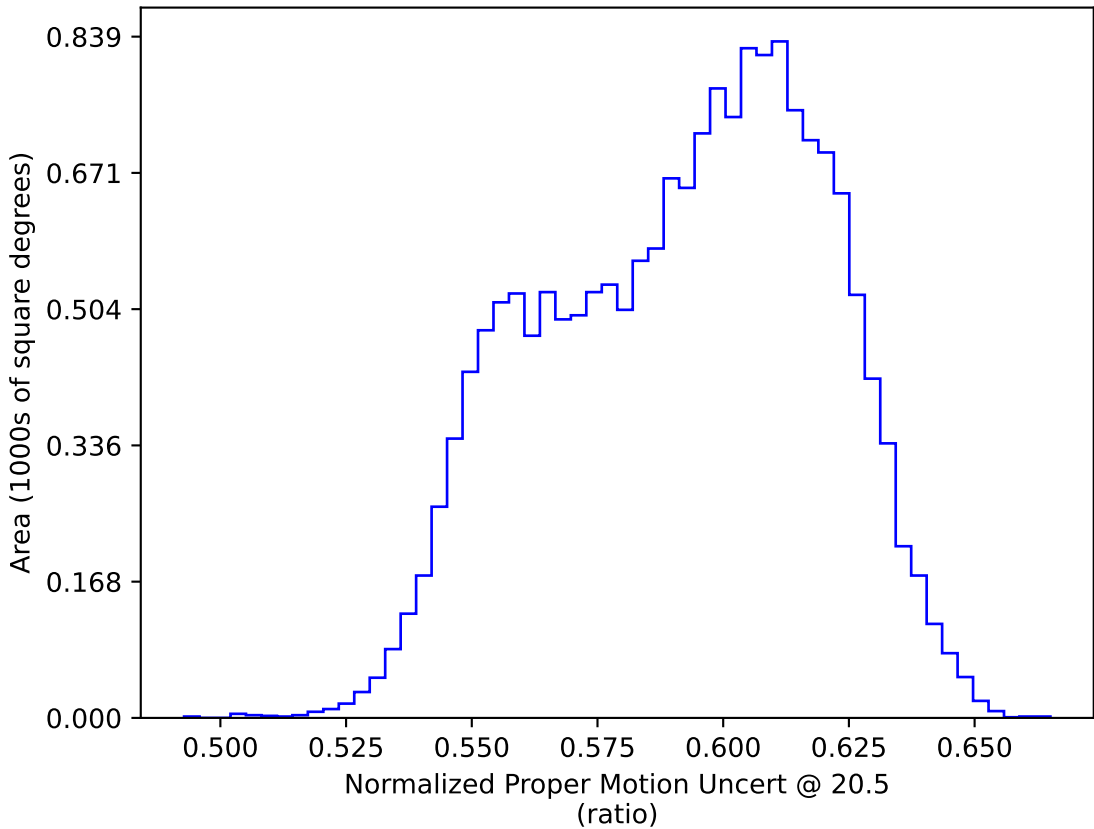
all_long_v3.4_10yrs WFD: Normalized Proper Motion Uncert @ 20.5
