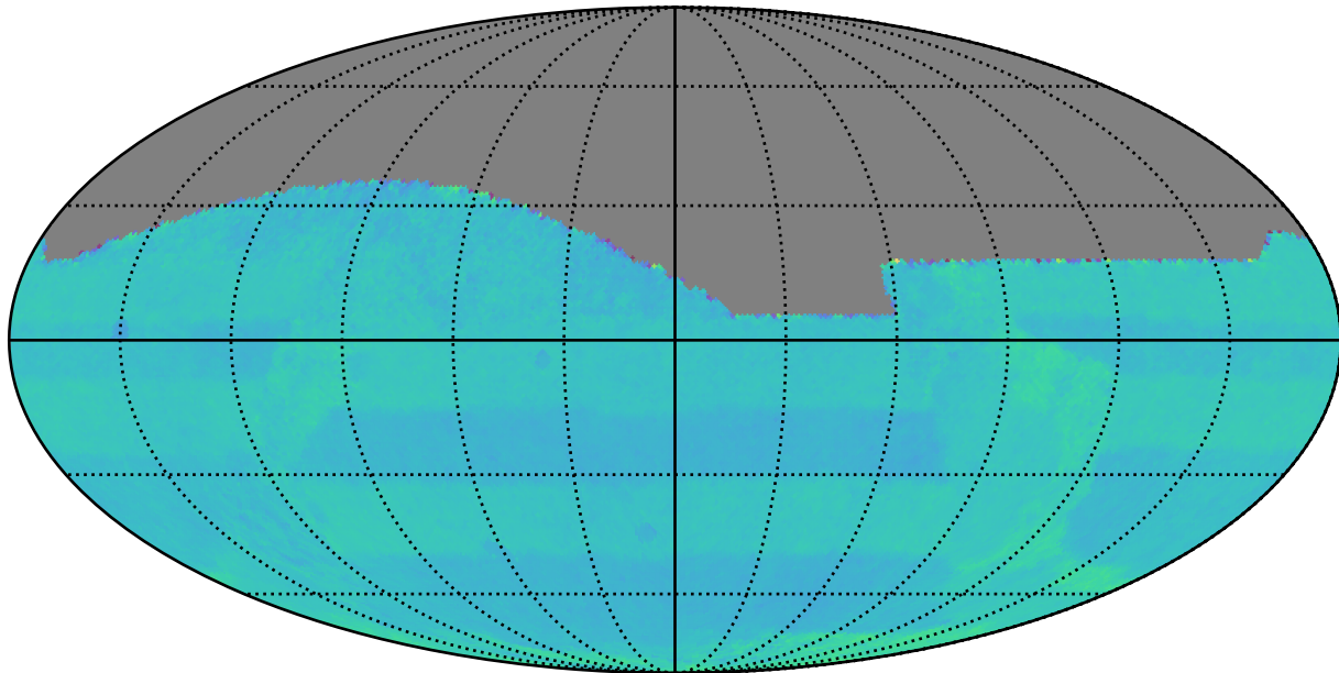
all_long_v3.4_10yrs All sky: Normalized Proper Motion Uncert @ 20.5
