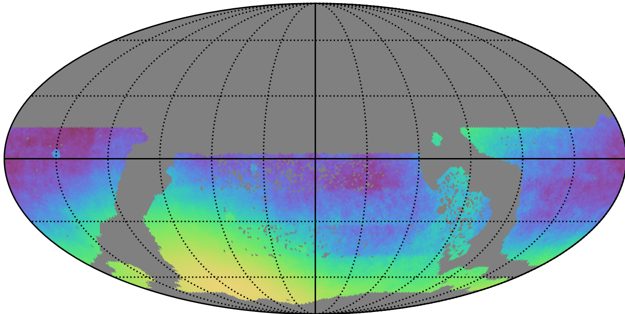
all_long_v3.4_10yrs WFD: Normalized Parallax Uncert @ 24.0
