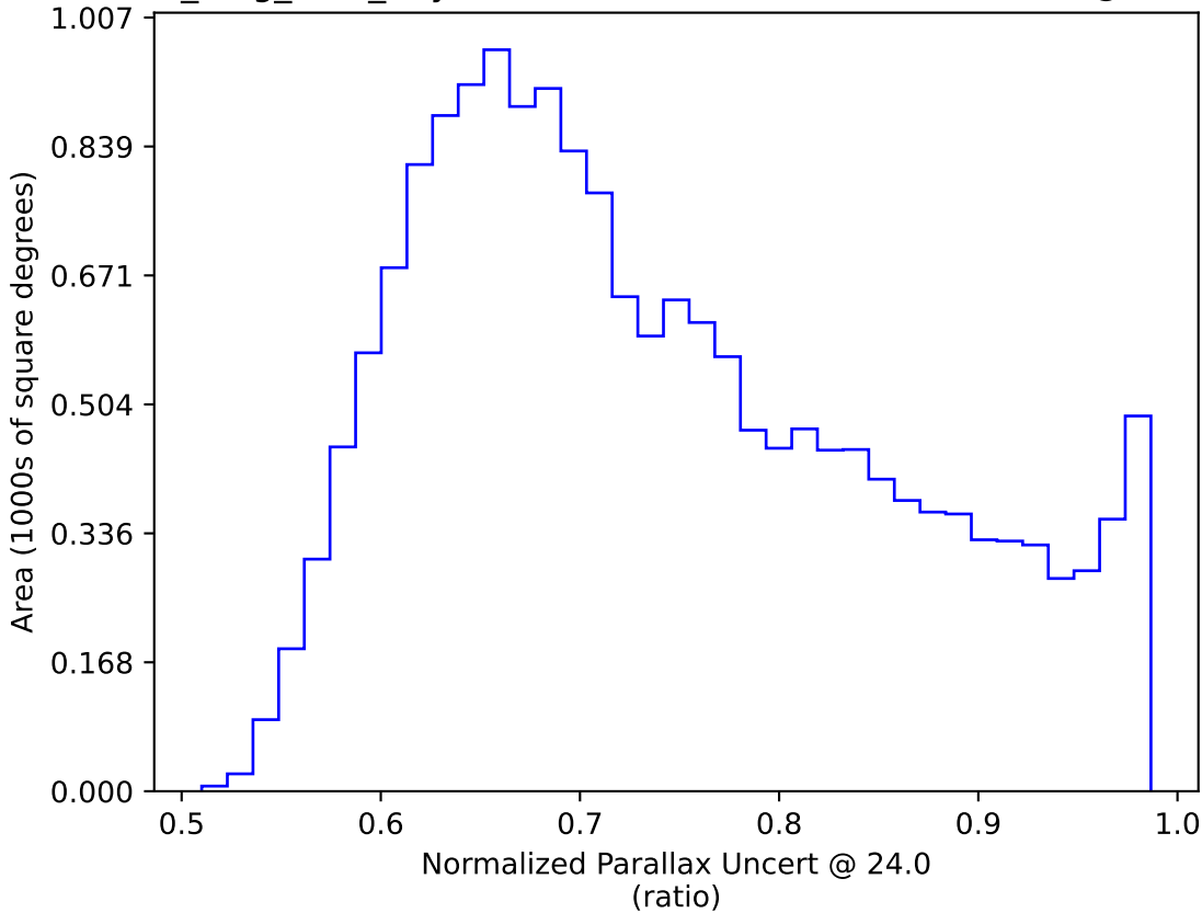
all_long_v3.4_10yrs WFD: Normalized Parallax Uncert @ 24.0
