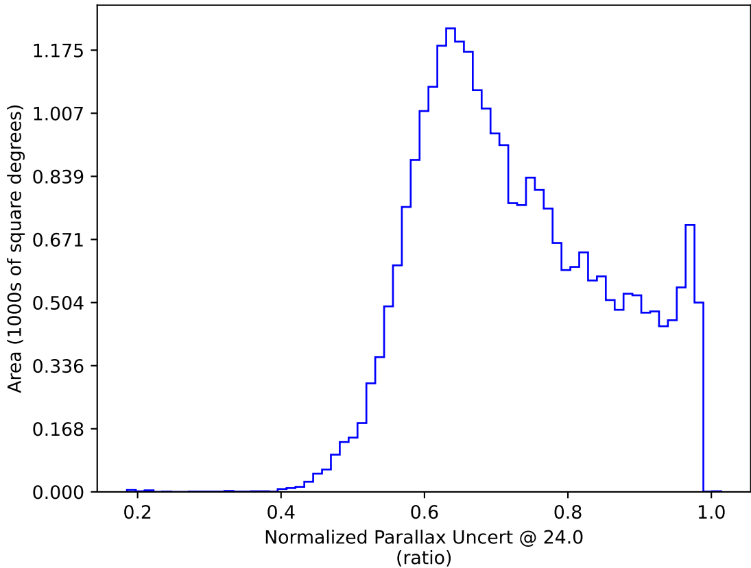
all_long_v3.4_10yrs All sky: Normalized Parallax Uncert @ 24.0
