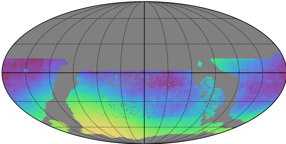
all_long_v3.4_10yrs WFD: Normalized Parallax Uncert @ 22.4
