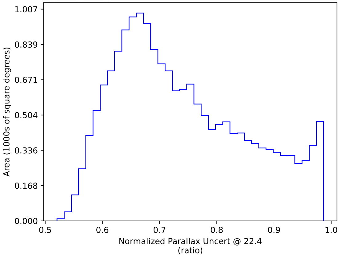
all_long_v3.4_10yrs WFD: Normalized Parallax Uncert @ 22.4
