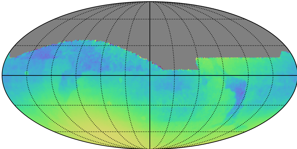
all_long_v3.4_10yrs All sky: Normalized Parallax Uncert @ 22.4
