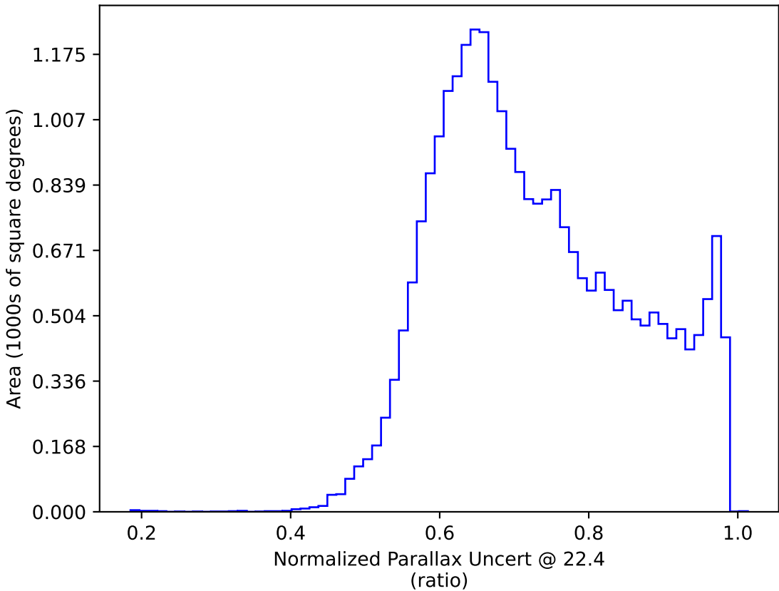
all_long_v3.4_10yrs All sky: Normalized Parallax Uncert @ 22.4
