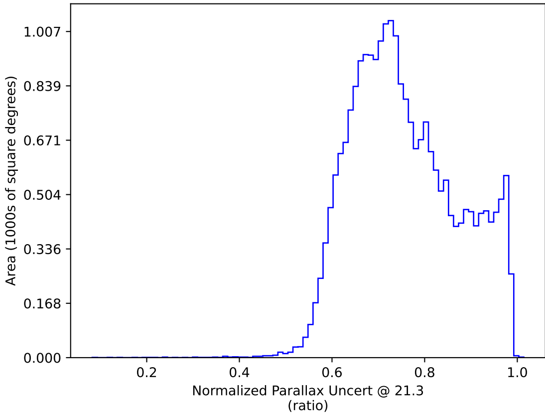
all_long_v3.4_10yrs All sky y band only: Normalized Parallax Uncert @ 21.3
