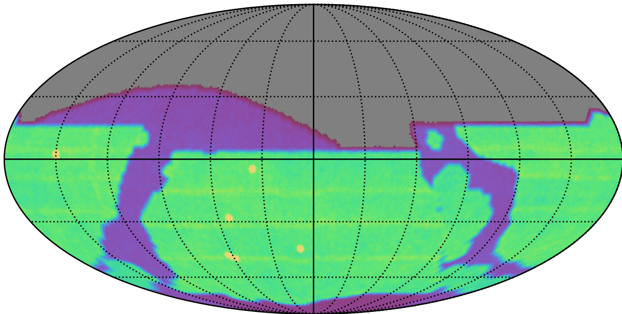
all_long_v3.4_10yrs All sky all bands: N Unique Nights
