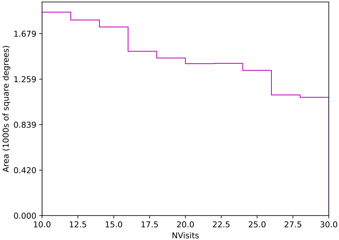
all_long_v3.4_10yrs Yr 3-4 z band: NVisits
