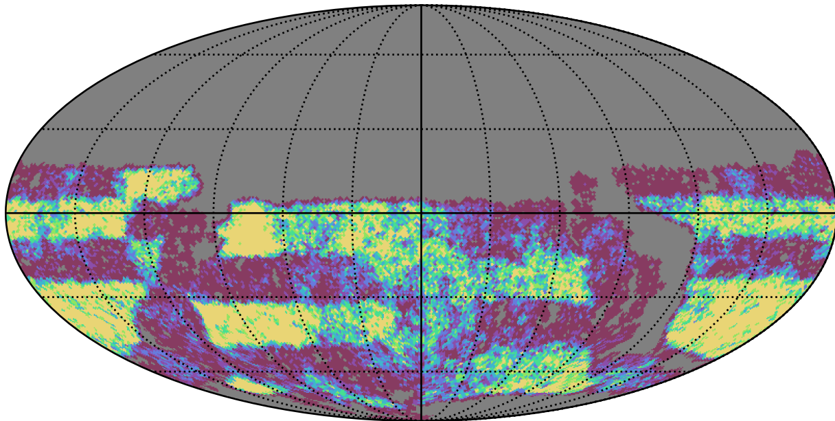
all_long_v3.4_10yrs Yr 3-4 u band: NVisits
