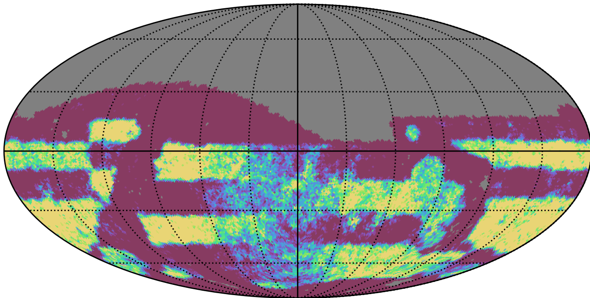
all_long_v3.4_10yrs Yr 3-4 r band: NVisits
