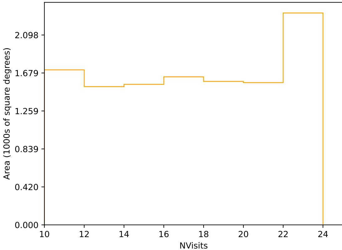
all_long_v3.4_10yrs Yr 3-4 r band: NVisits
