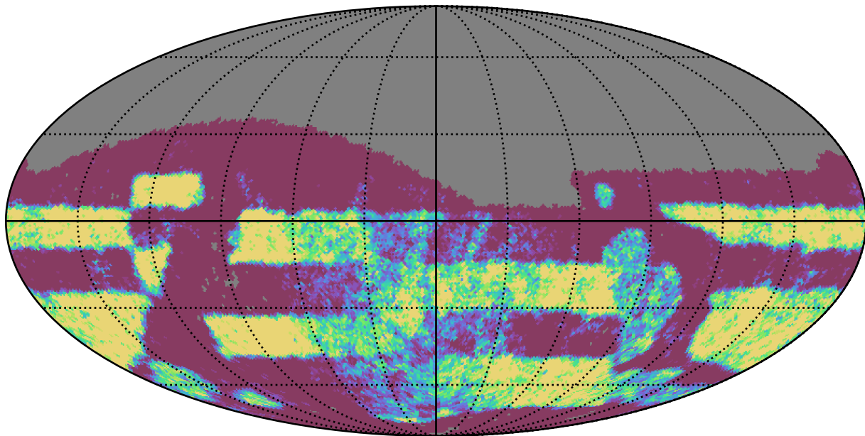
all_long_v3.4_10yrs Yr 3-4 i band: NVisits
