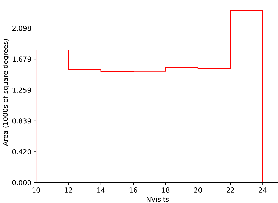
all_long_v3.4_10yrs Yr 3-4 i band: NVisits
