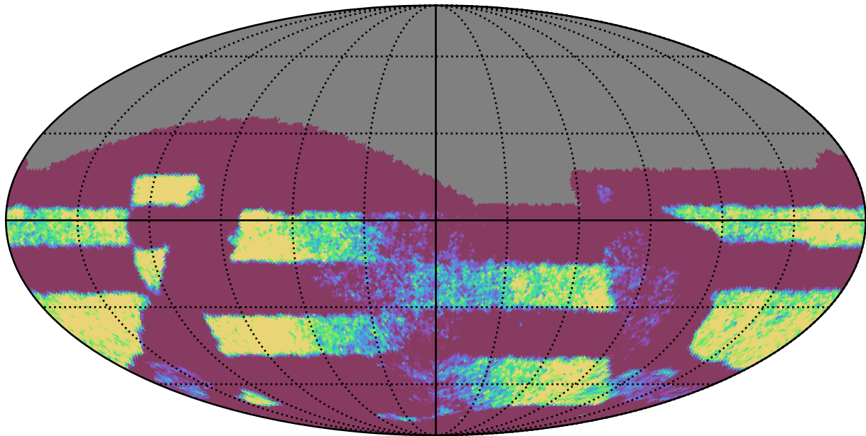
all_long_v3.4_10yrs Yr 3-4 all bands: NVisits
