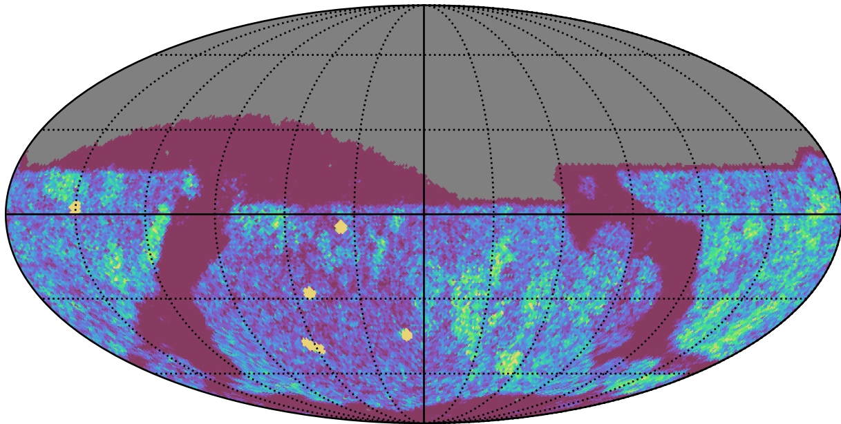
all_long_v3.4_10yrs Yr 1 z band: NVisits
