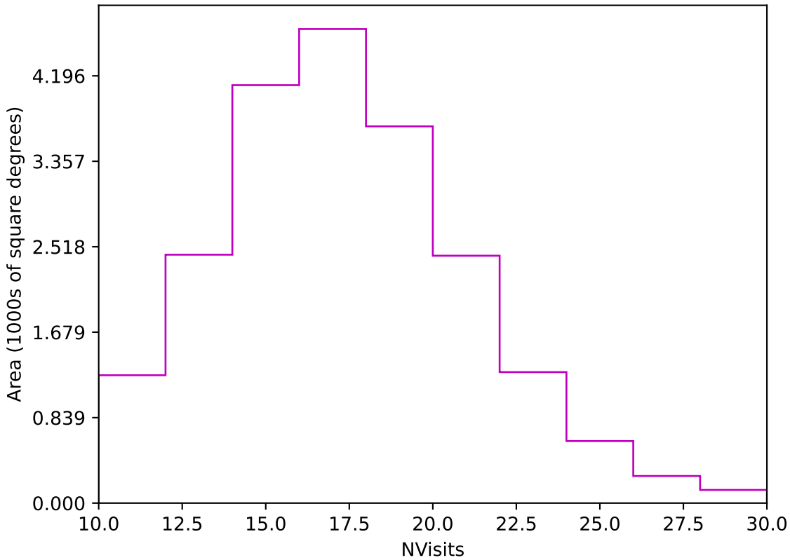
all_long_v3.4_10yrs Yr 1 z band: NVisits
