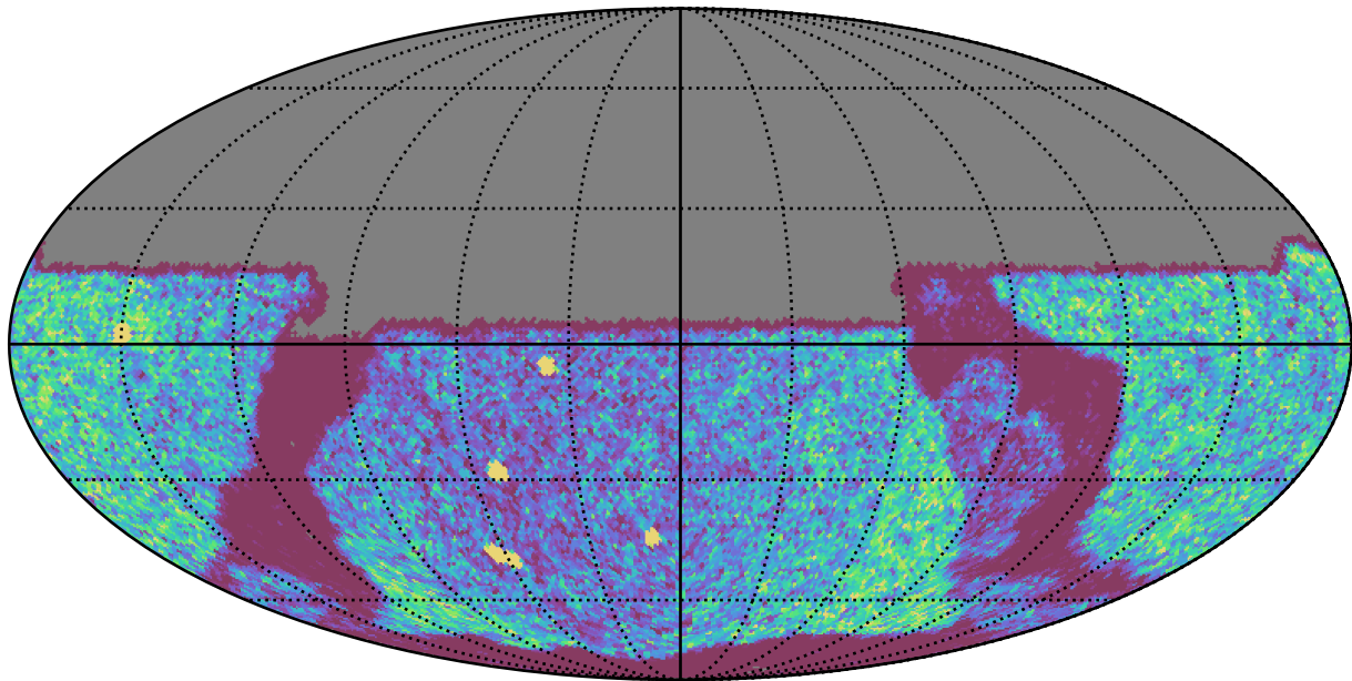
all_long_v3.4_10yrs Yr 1 y band: NVisits
