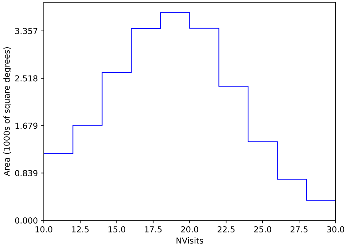
all_long_v3.4_10yrs Yr 1 y band: NVisits
