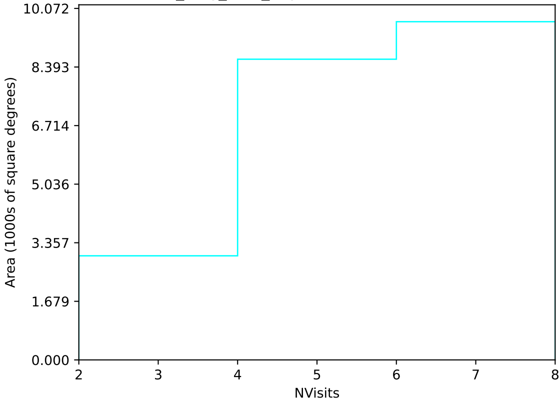
all_long_v3.4_10yrs Yr 1 u band: NVisits
