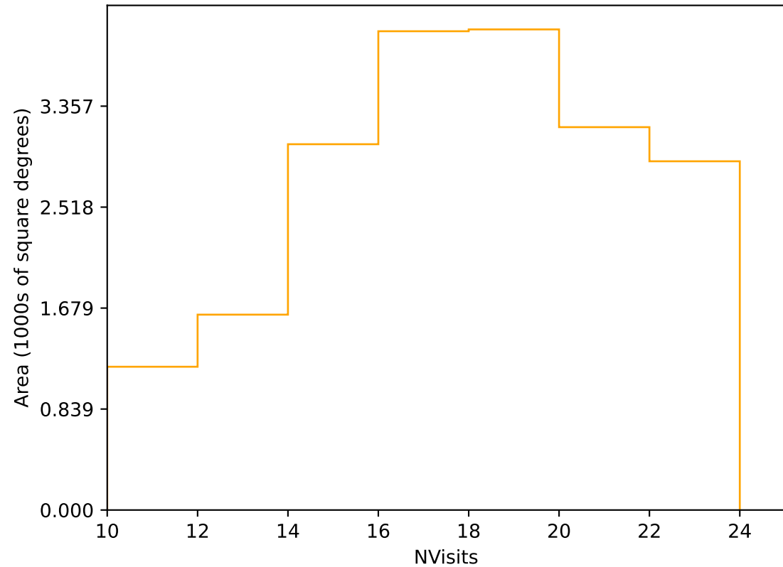
all_long_v3.4_10yrs Yr 1 r band: NVisits
