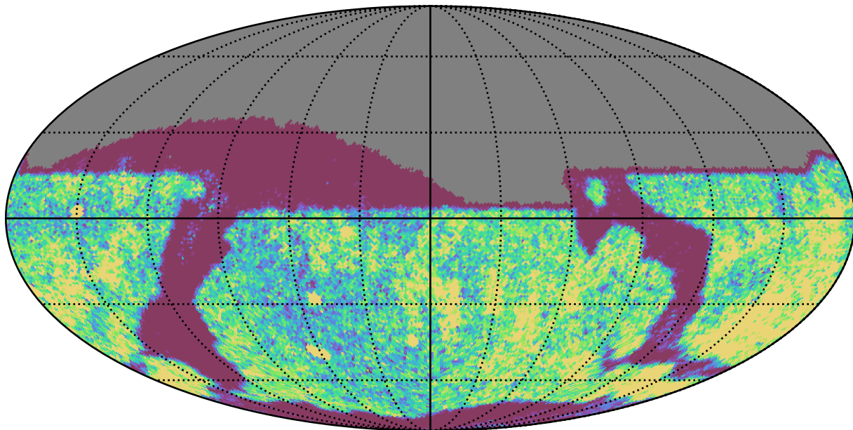
all_long_v3.4_10yrs Yr 1 i band: NVisits
