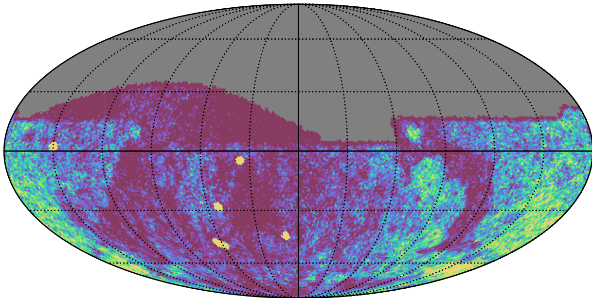
all_long_v3.4_10yrs Yr 1 g band: NVisits
