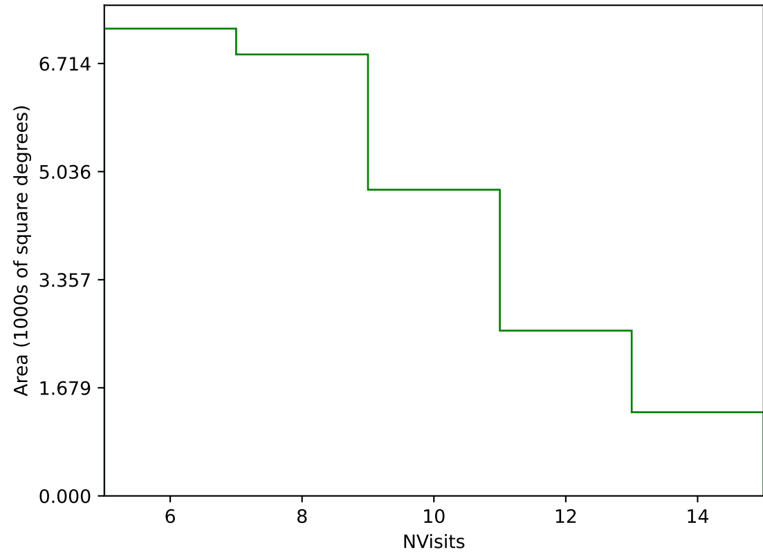
all_long_v3.4_10yrs Yr 1 g band: NVisits
