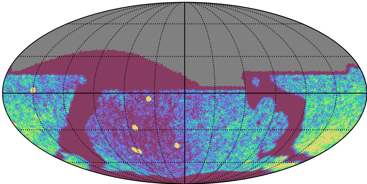
all_long_v3.4_10yrs Yr 1 all bands: NVisits
