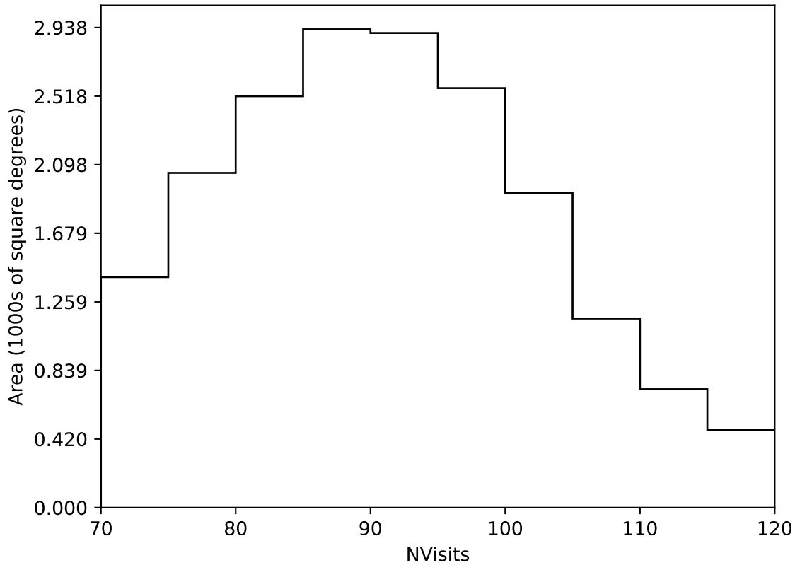
all_long_v3.4_10yrs Yr 1 all bands: NVisits
