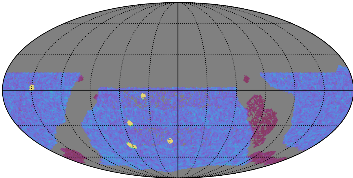
all_long_v3.4_10yrs WFD y band: NVisits
