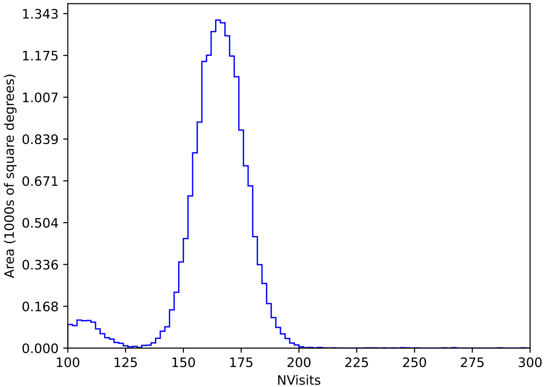
all_long_v3.4_10yrs WFD y band: NVisits
