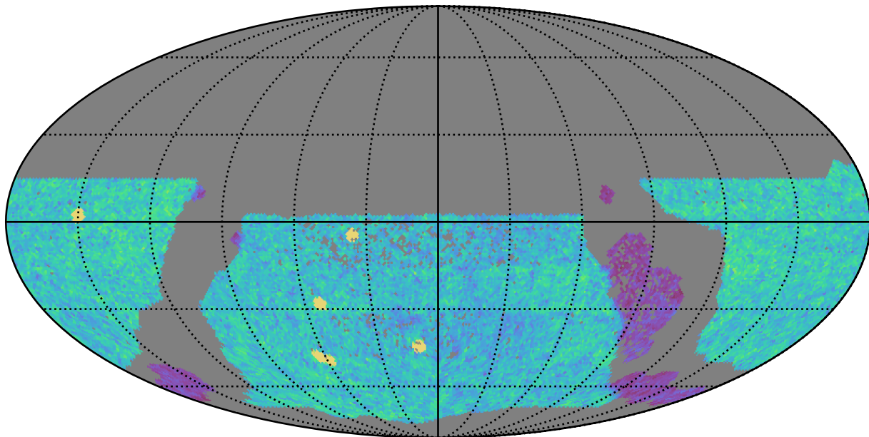
all_long_v3.4_10yrs WFD u band: NVisits
