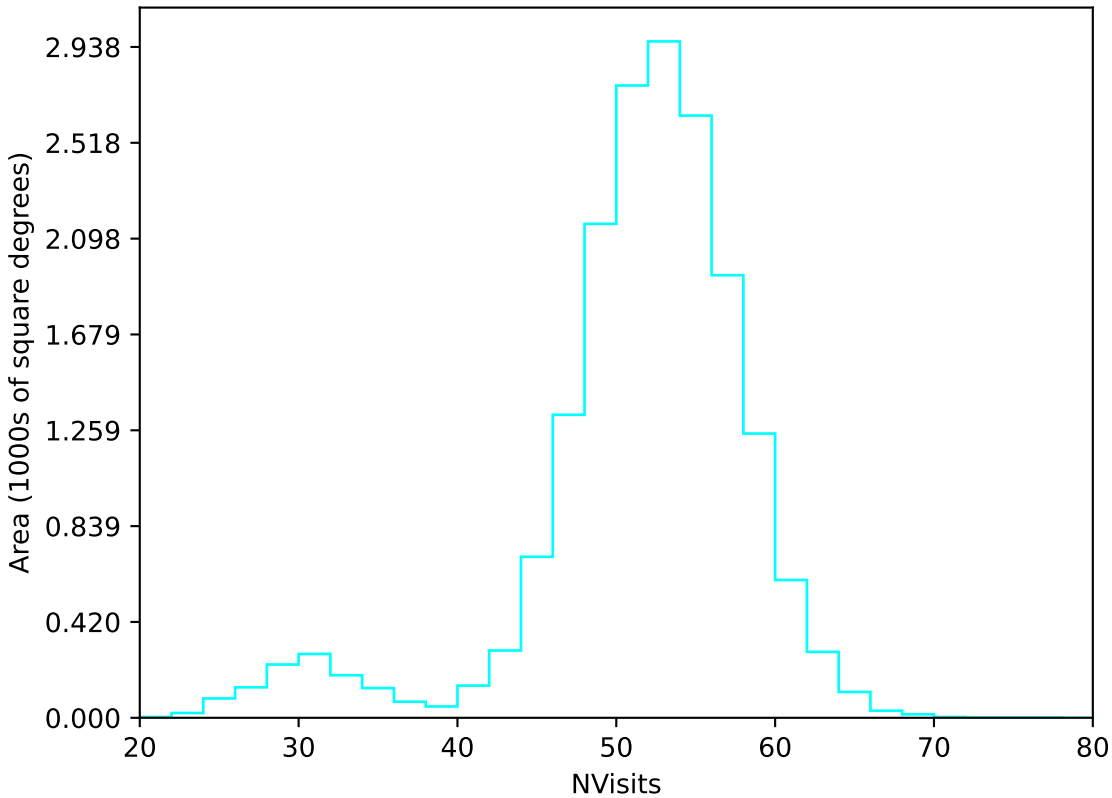
all_long_v3.4_10yrs WFD u band: NVisits
