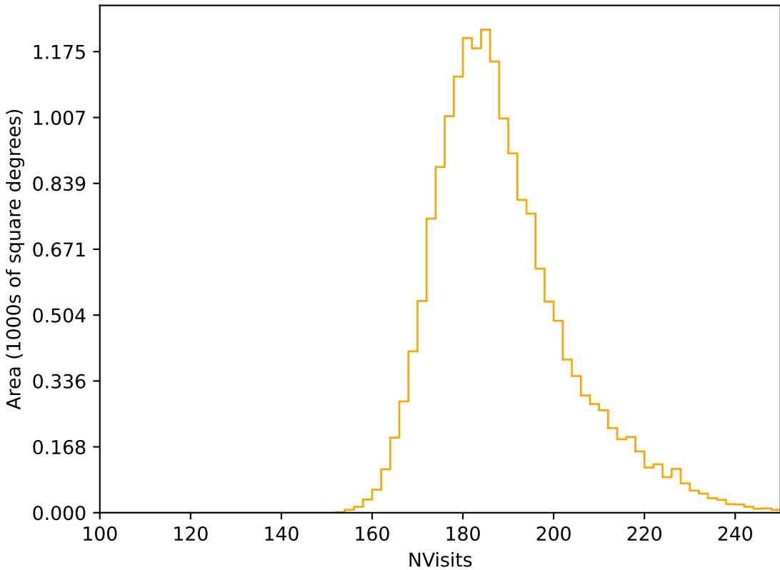
all_long_v3.4_10yrs WFD r band: NVisits
