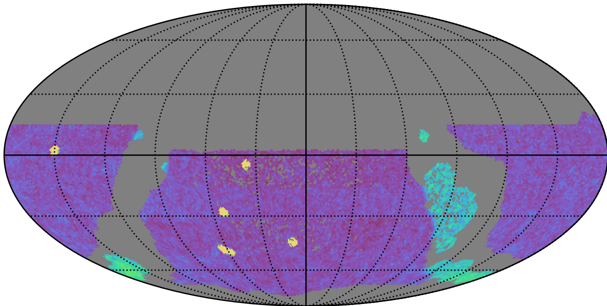
all_long_v3.4_10yrs WFD g band: NVisits
