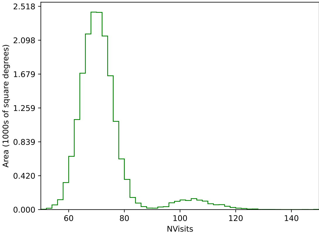
all_long_v3.4_10yrs WFD g band: NVisits
