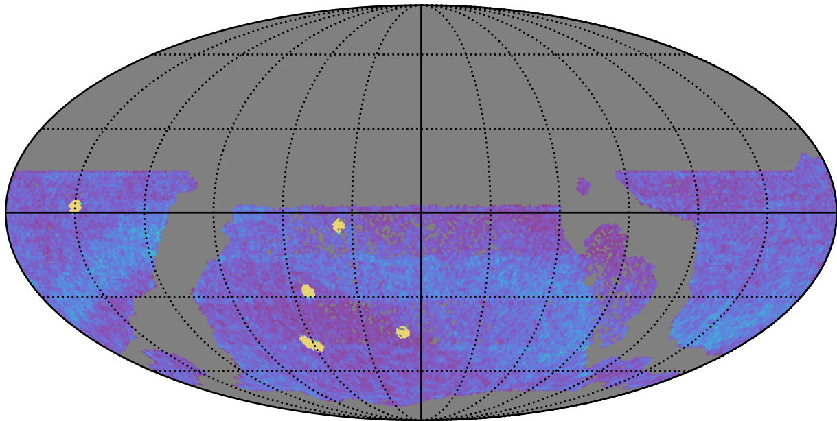
all_long_v3.4_10yrs WFD all bands: NVisits
