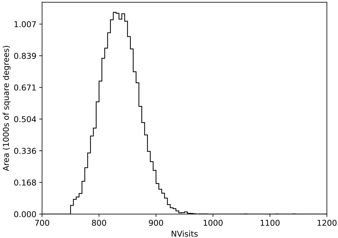
all_long_v3.4_10yrs WFD all bands: NVisits
