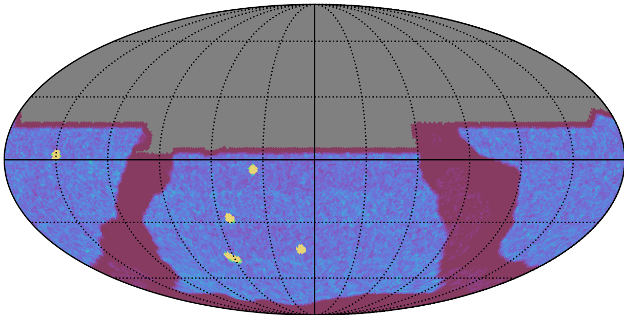
all_long_v3.4_10yrs All sky y band: NVisits
