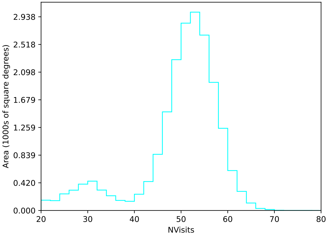
all_long_v3.4_10yrs All sky u band: NVisits
