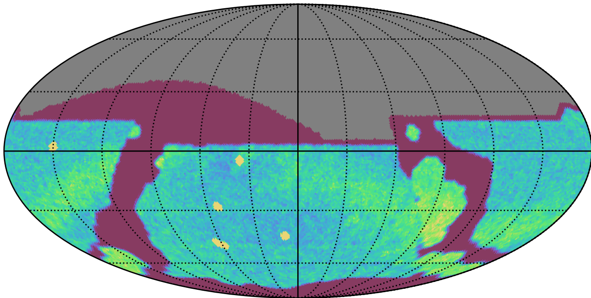
all_long_v3.4_10yrs All sky r band: NVisits
